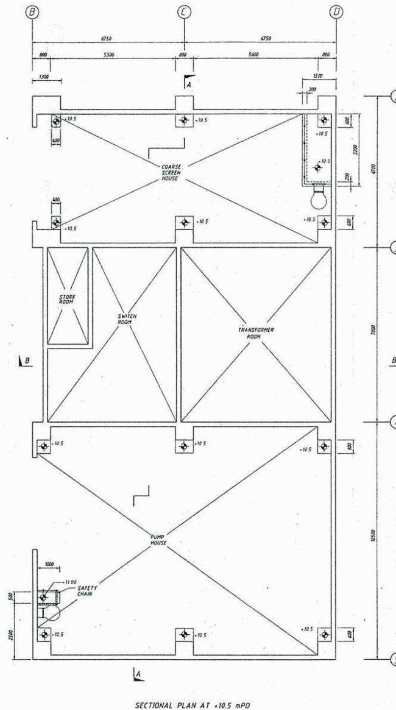
Figure 2: Sewage Pumping Station and Equalization Tanks - Plans
